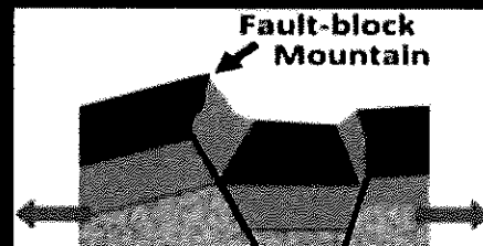
Fault-block
